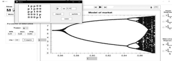
Fig. 2. Model application window for general view market model
