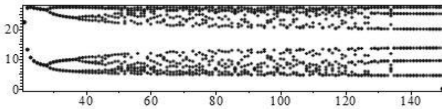
Fig. 7. The bifurcation diagram of dependence of quantity product x_1 on n at \delta = 0.2 .
