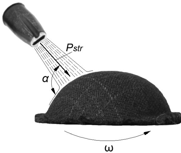
Figure 1 Theme of technological process of hydro-jet forming
