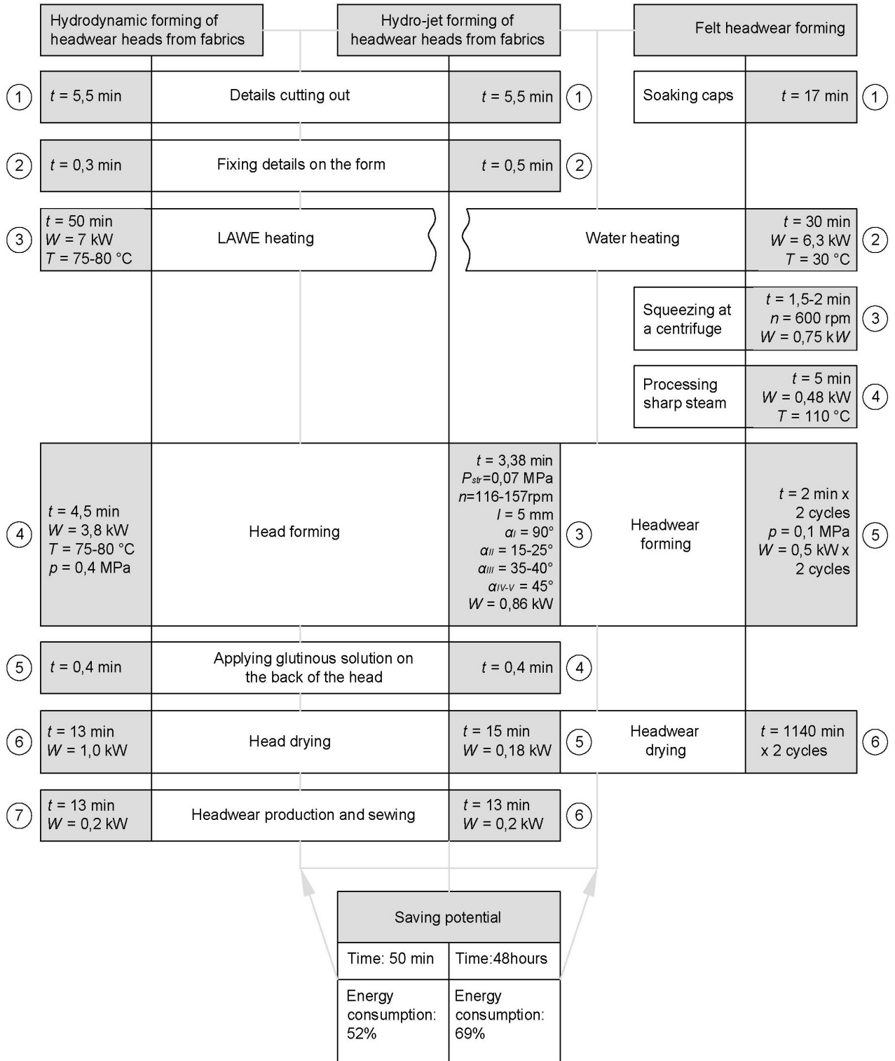
Figure 3 Saving potential developed hydro-jet technology in comparison with hydrodynamic forming and felt forming
