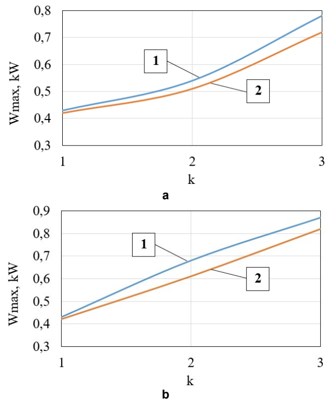
Figure 2 Graphic dependencies of changes the maximum energy consumption W_{max} from the factor, that takes into account a number of material layers k : 1 – press equipment with a standard flywheel; 2 – press equipment with a new flywheel design; a – coat fabric; b – costume fabric
