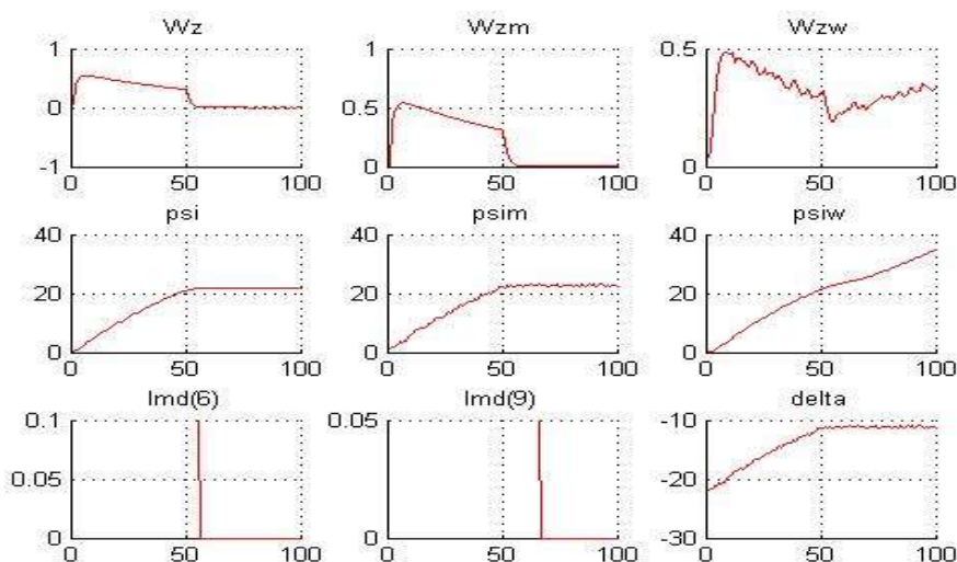
Figure 6 – Detection of angle motion control channel failure
